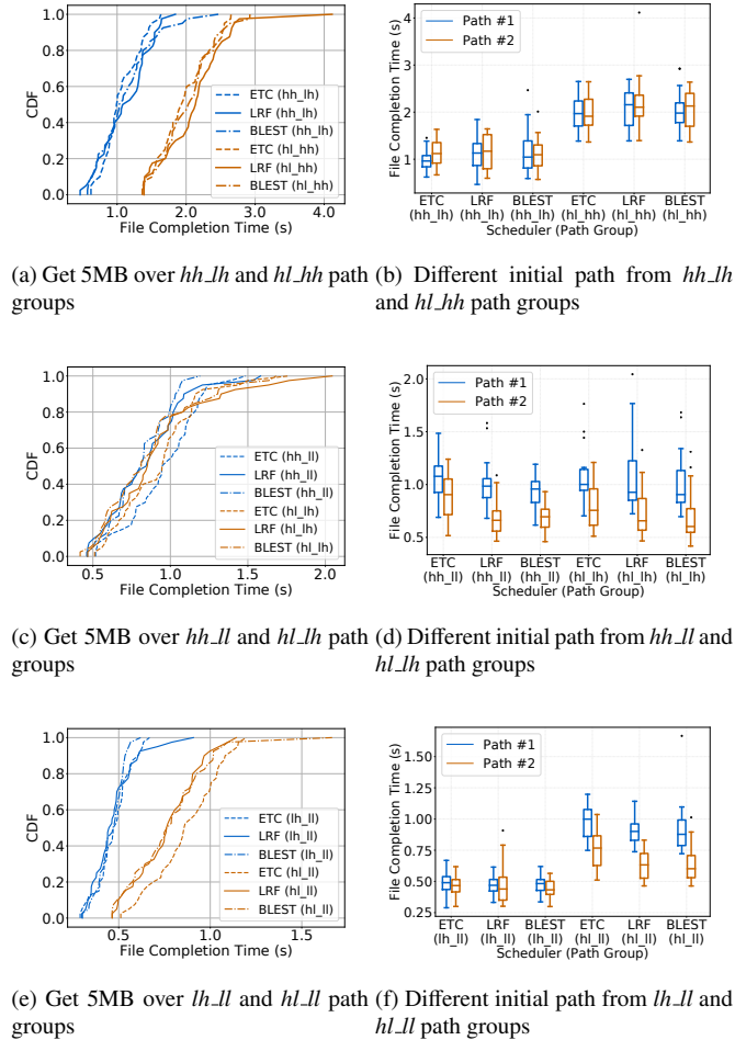
Figure 7: Get 5MB using h2quic with TLS over six types of heterogeneous paths.
