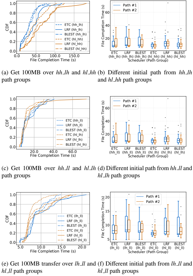
Figure 6: Get 100MB using h2quic with TLS over six types of heterogeneous paths. ETC's performance is better than LRF and BLEST.
