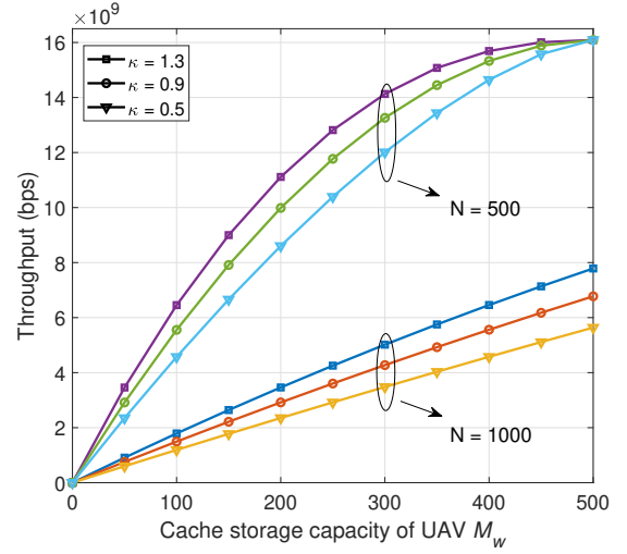
Fig. 11. Network throughput using the proposed CMARL algorithm with different cache storage capacities.
