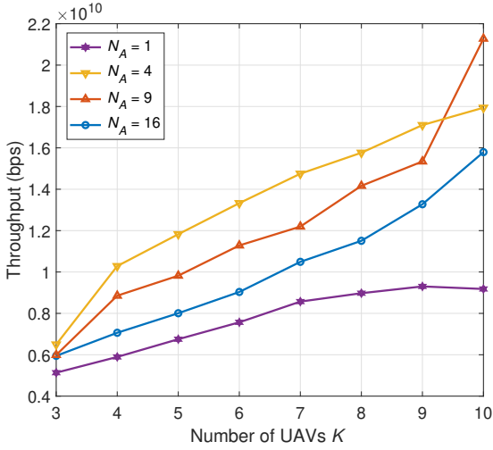
Fig. 9. Network throughput using the proposed CMARL algorithm with different numbers cooperative regions.
