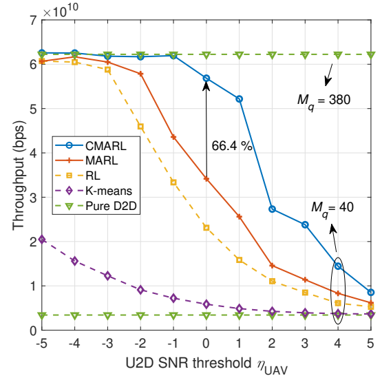
Fig. 4. Network throughput versus U2D SNR threshold.
