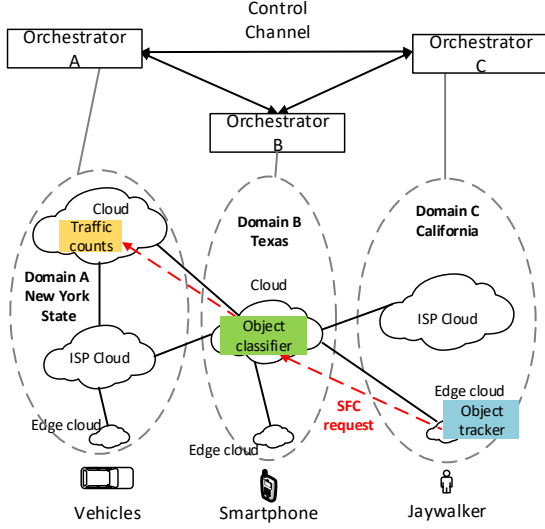
Figure 1: An example for SFC in 3-tier (cloud-ISP-edge) architecture
