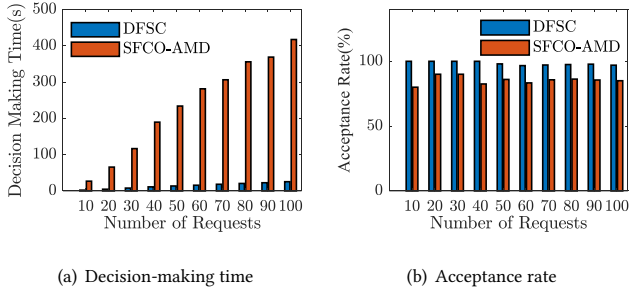
Figure 7: The comparison of decision-making time and acceptance rate
