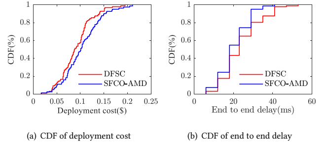
Figure 8: CDF of deployment cost and delay
